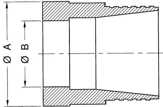
Core Bits with External Thread Connections
